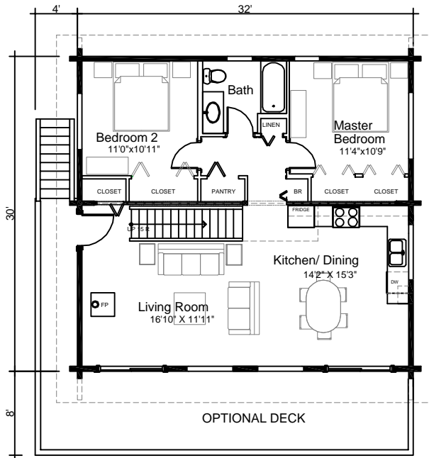
MAIN FLOOR
