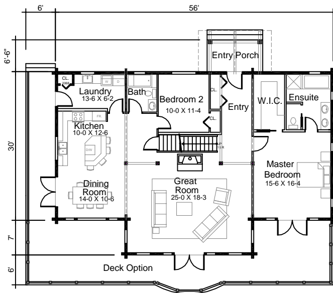
MAIN FLOOR
