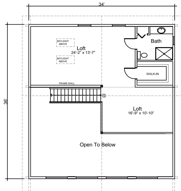
LOFT FLOOR
