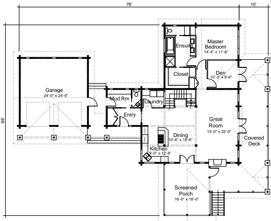
MAIN FLOOR
